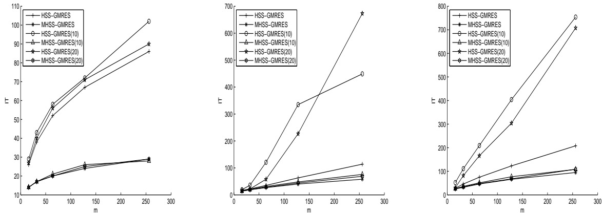
Figure 2: Pictures of IT versus m for HSS- and MHSS-preconditioned GMRES(10), GMRES(20) and GMRES methods; left: Example 4.1, middle: Example 4.2, and right: Example 4.3.
