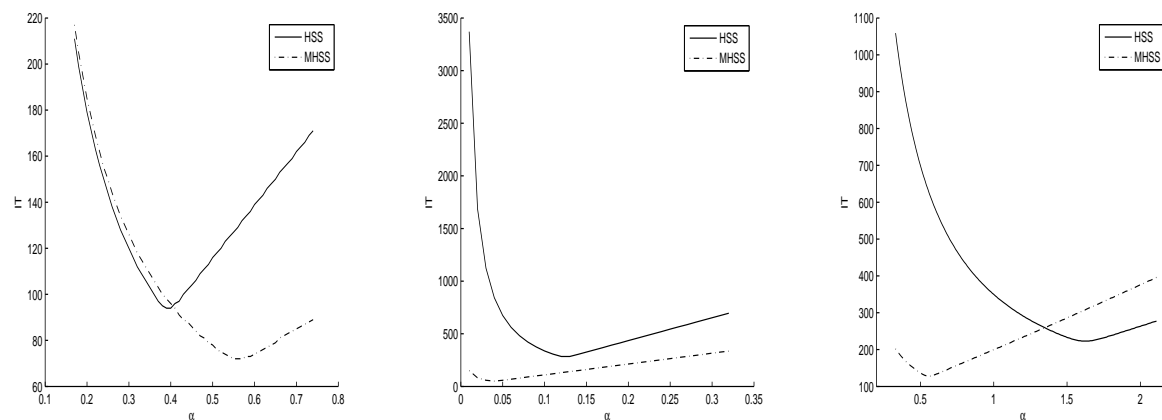
Figure 1: Pictures of IT versus \alpha for HSS and MHSS iteration methods; left: Example 4.1, middle: Example 4.2, and right: Example 4.3.
